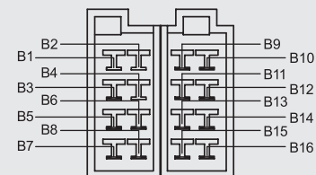
ISO CONNECTORS (HARNESS)
