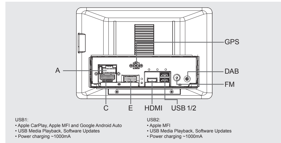
16 PIN CONNECTOR (DEVICE BACKSIDE)
